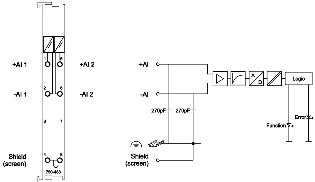
Figure 5: Schematic Diagram
