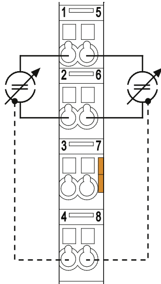
Figure 10: Connection Example 750-483
