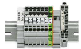
This delta jumper has been specially developed to create a delta configuration and is used on motor terminal boards equipped with rail-mount terminal blocks TOPJOB® S.
